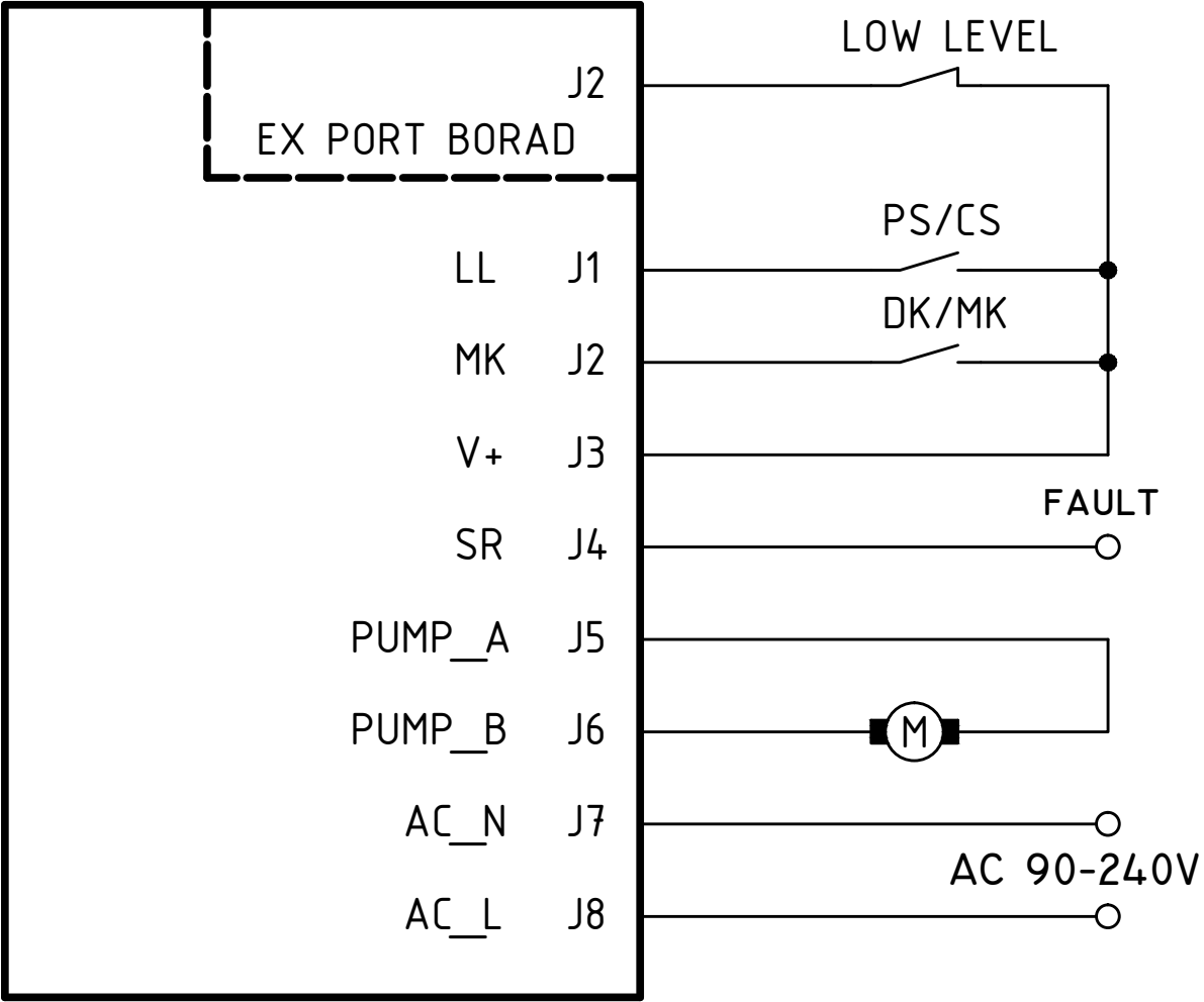
UC-1AC CONNECTION DIAGRAM
